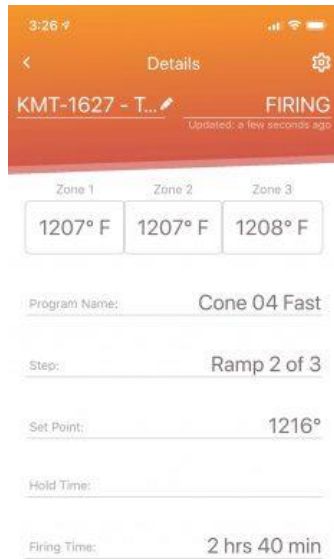
KilnLink App
